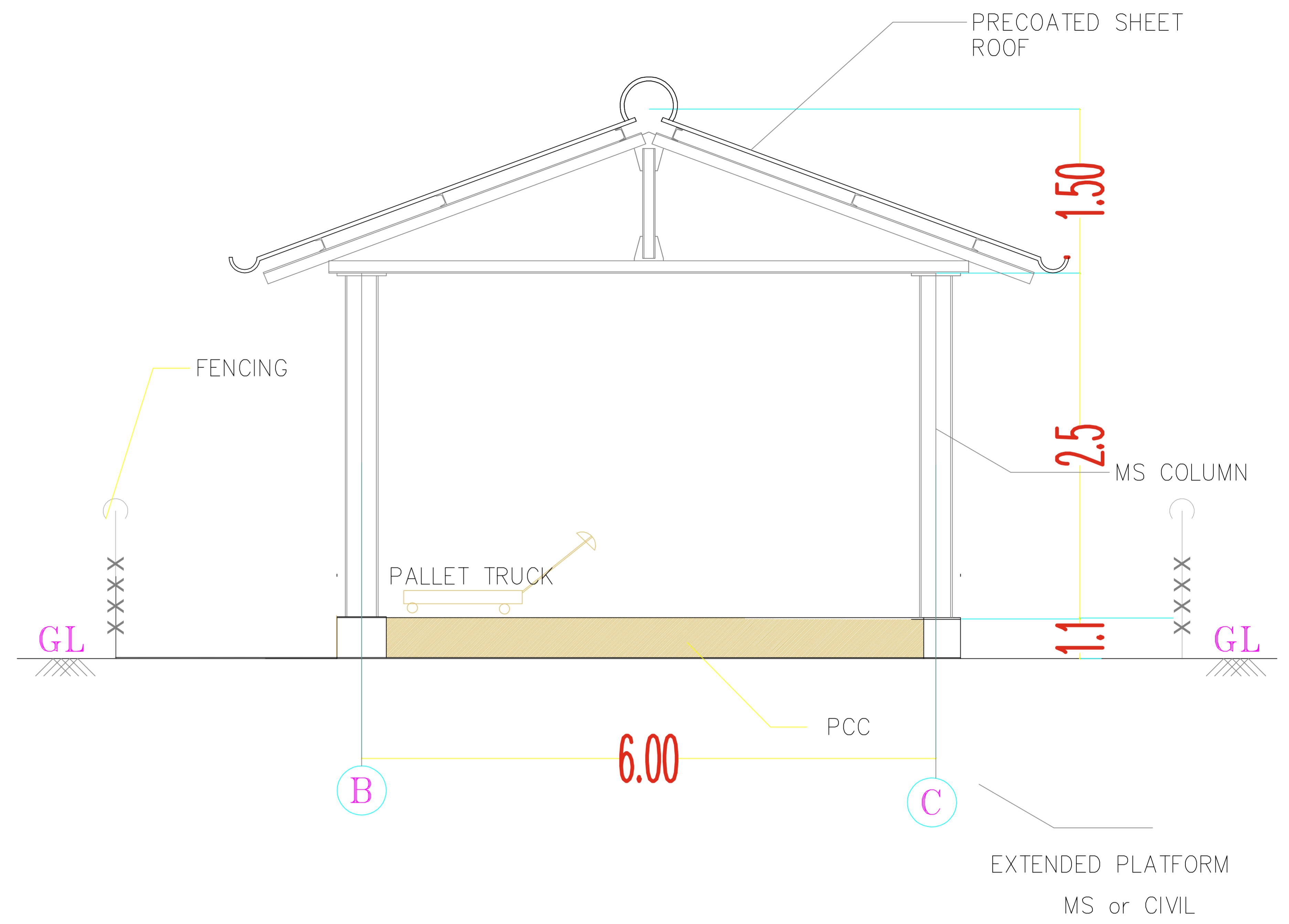
CROSS SECTION
