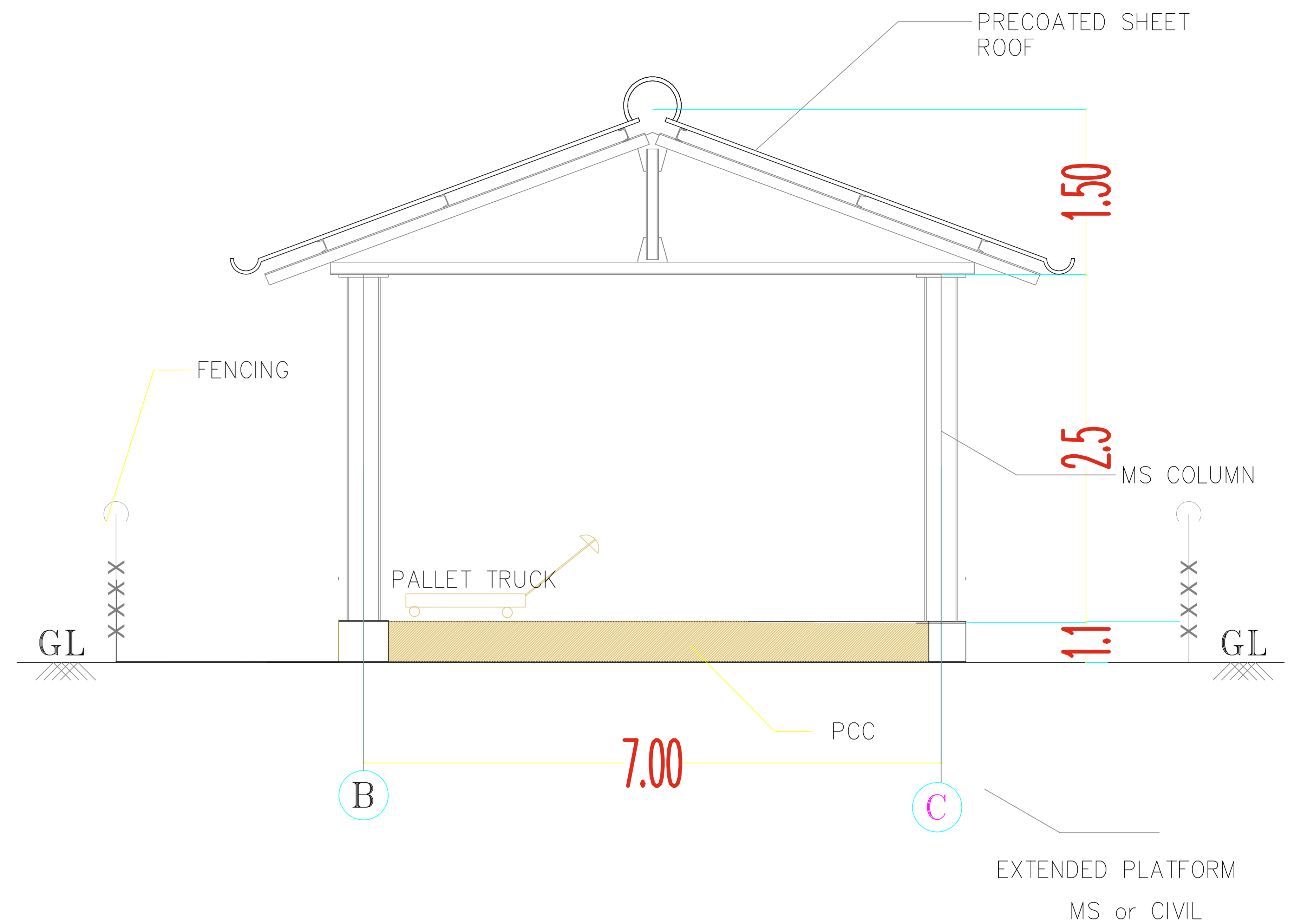
CROSS SECTION
